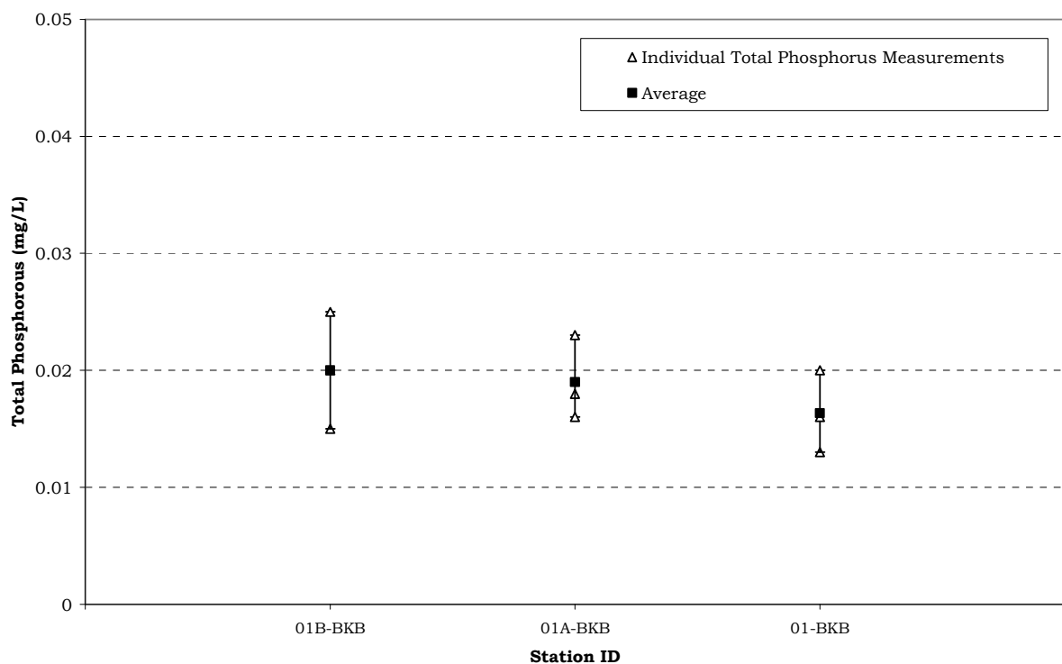
Figure 6. Total Phosphorus Statistics for Black Brook June 20 - August 20, 2010 NHDES VRAP
