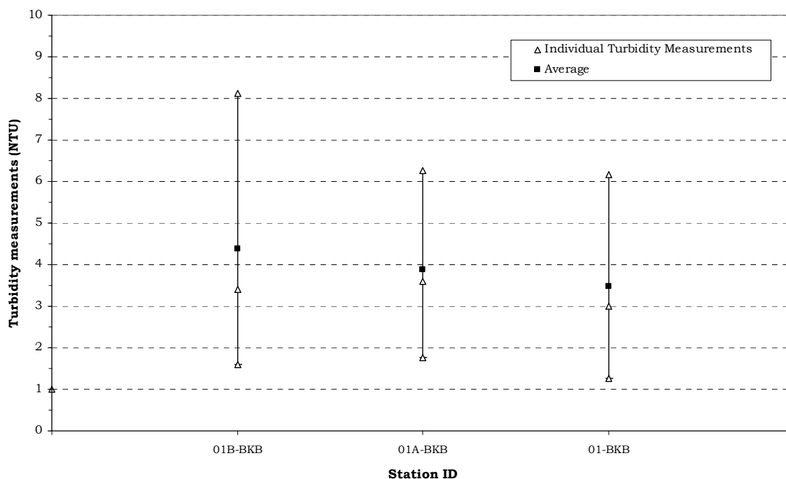
Figure 3. Turbidity Statistics for Black Brook June 27 - August 20, 2010, NHDES VRAP
