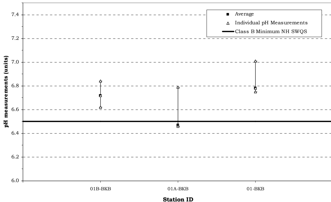
Figure 2. pH Statistics for Black Brook June 27 - August 20, 2010, NHDES VRAP
