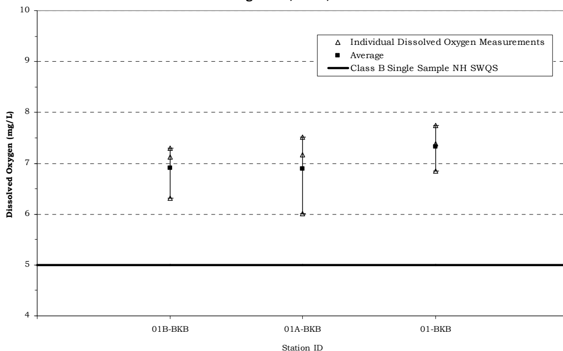
Figure 1. Dissolved Oxygen Concentration Statistics for Black Brook June 27 - August 20, 2010, NHDES VRAP
