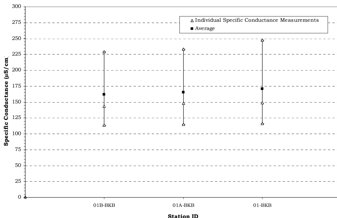
Figure 4. Specific Conductance Statistics for Black Brook June 27 - August 20, 2010, NHDES VRAP
