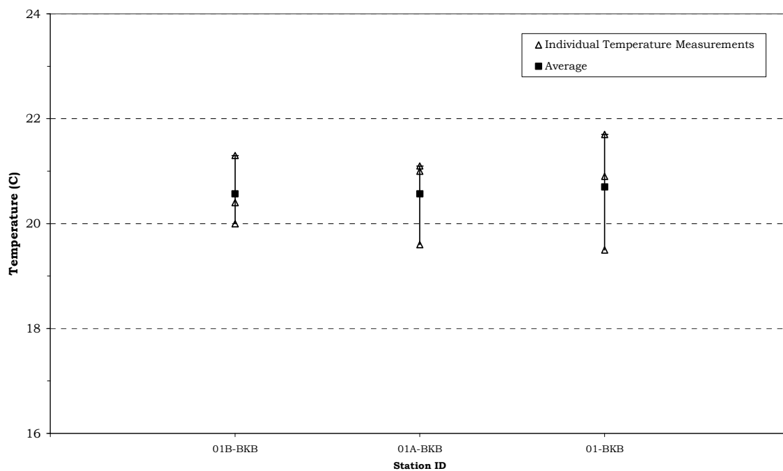
Figure 5. Water Temperature Statistics for Black Brook June 20 - August 20, 2010, NHDES VRAP
