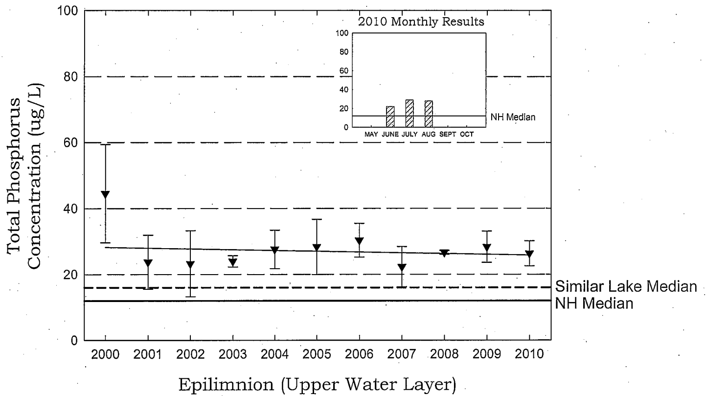
Figure 3. Monthly and Historical Total Phosphorus Data.
